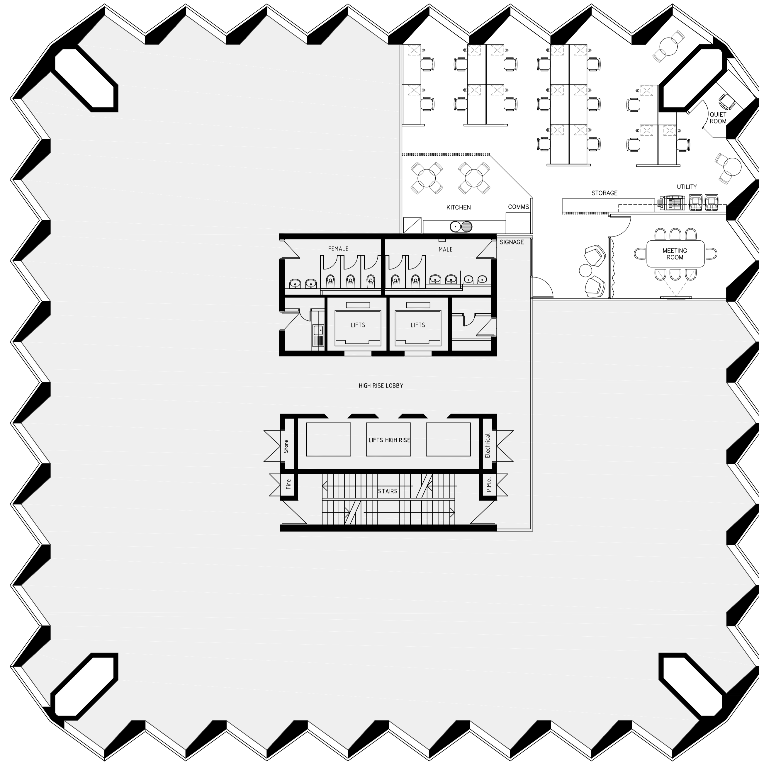
01 PROPOSED GENERAL ARRANGEMENT SCALE 1:100
